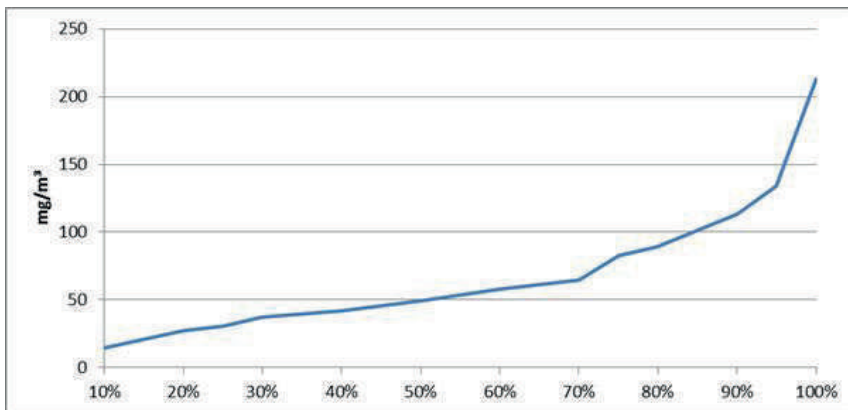
Fig. 1: Overview of the calculated THF measured values for PVC-Cold-Welding (mg/m 3 )
